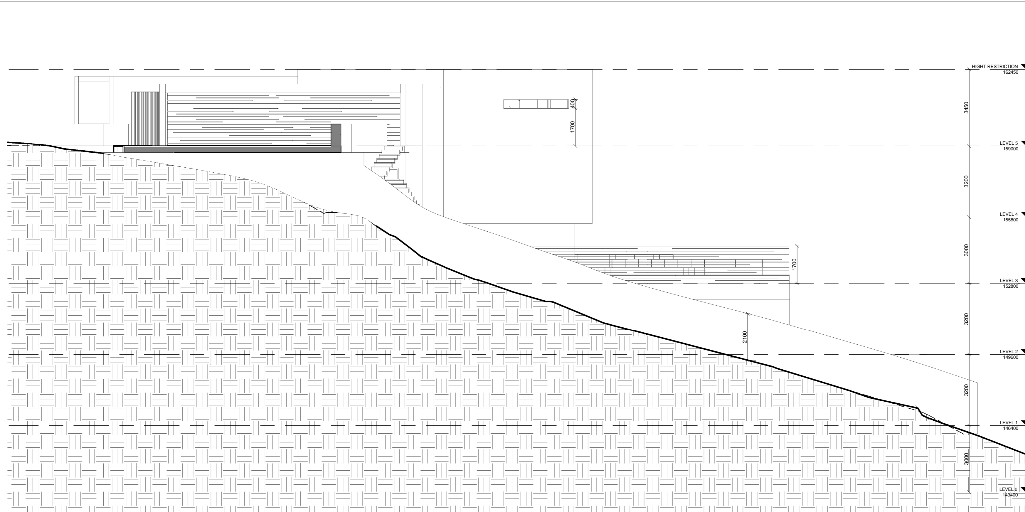
NORTH ELEVATION 1 : 100
